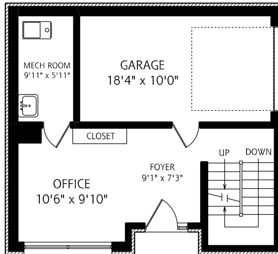
GROUND FLOOR 415 SQUARE FEET
