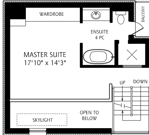
THIRD FLOOR 470 SQUARE FEET
